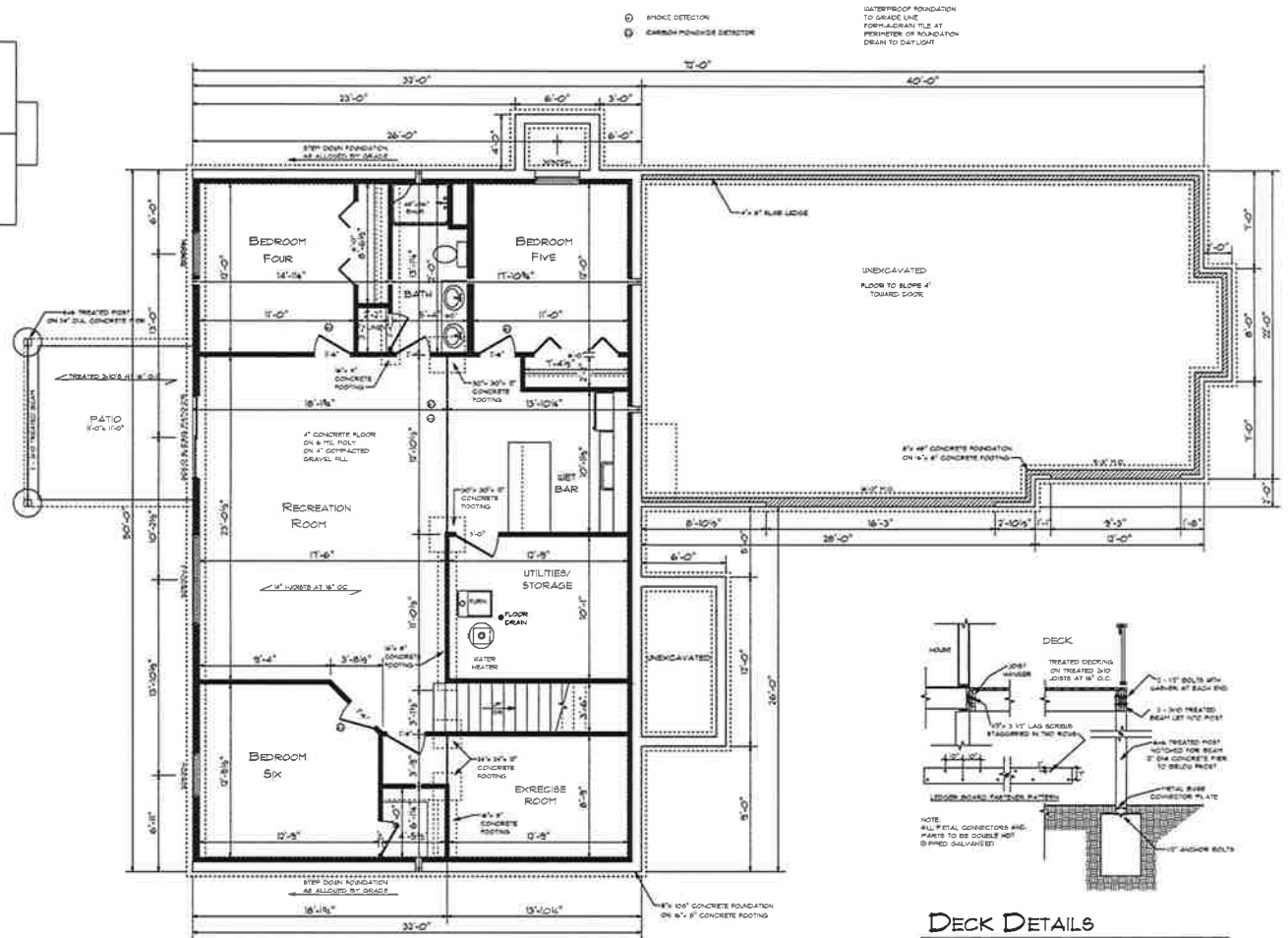
FOUNDATION & LOWER LEVEL FLOOR PLAN
