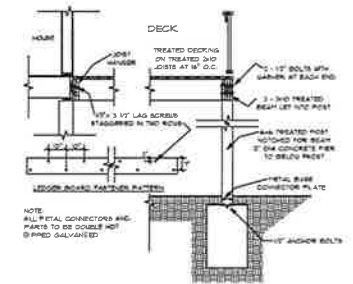
DECK DETAILS
