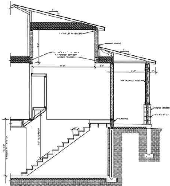
STAIR SECTION
